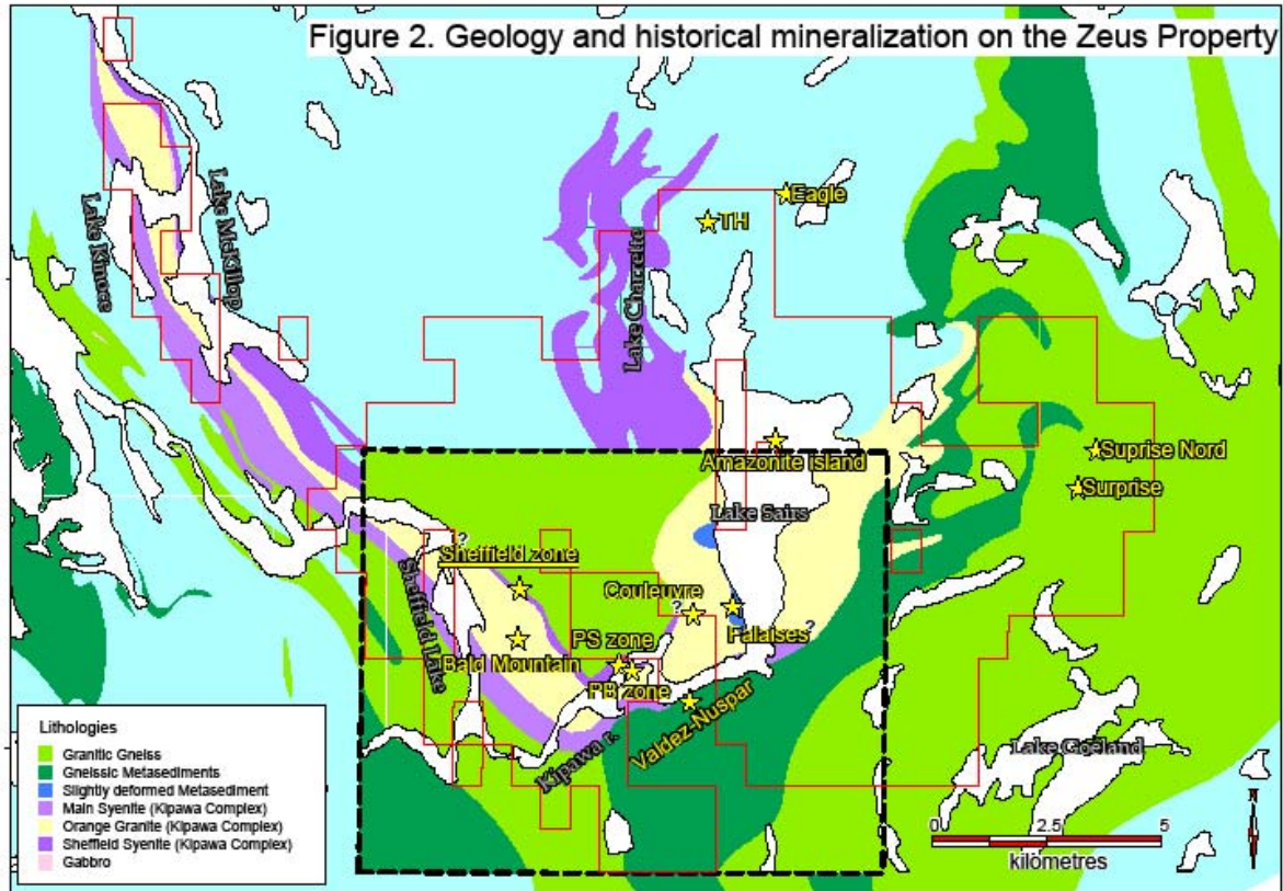
Figure 2. Geology and historical mineralization on the Zeus property
